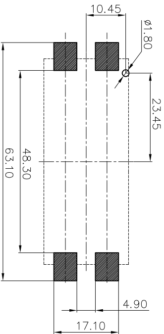
PCB Layout Diagram Top View
