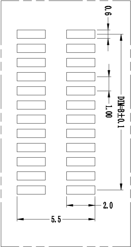
PCB Layout
