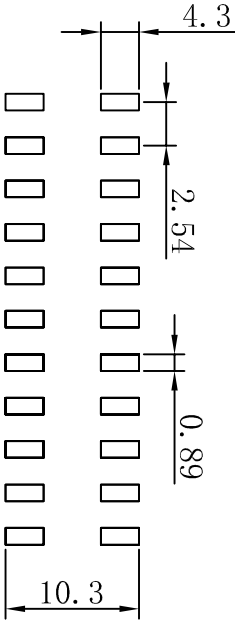
PCB LAYOUT
