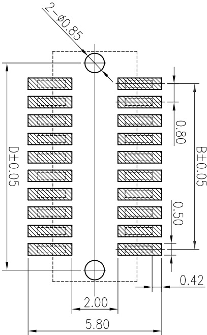
RECOMMENDED PCB PATTERN DIM. TOLERANCE : ±0.05
