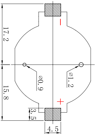
PCB Layout Diagram Top View
