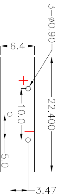
PCB Layout Diagram Top View
